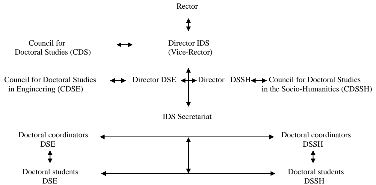
Organisational chart of DJUG Doctoral School
